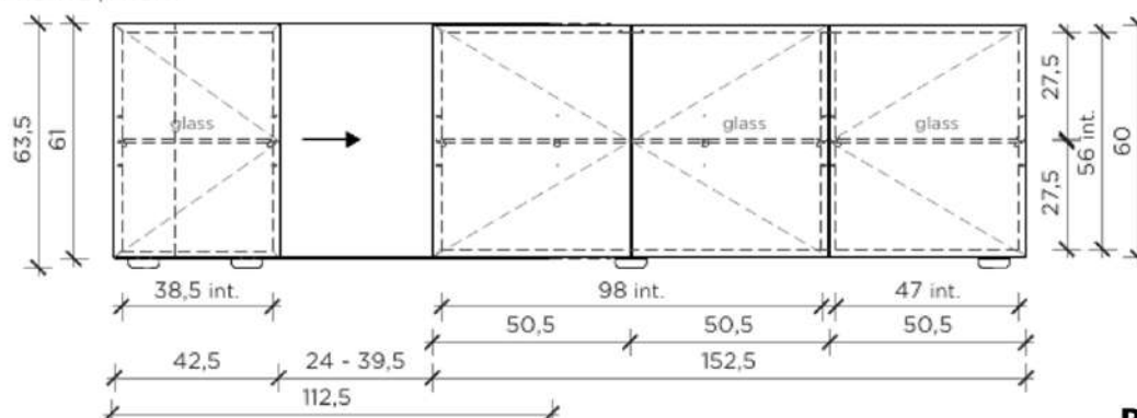
FRONTE | FRONT
